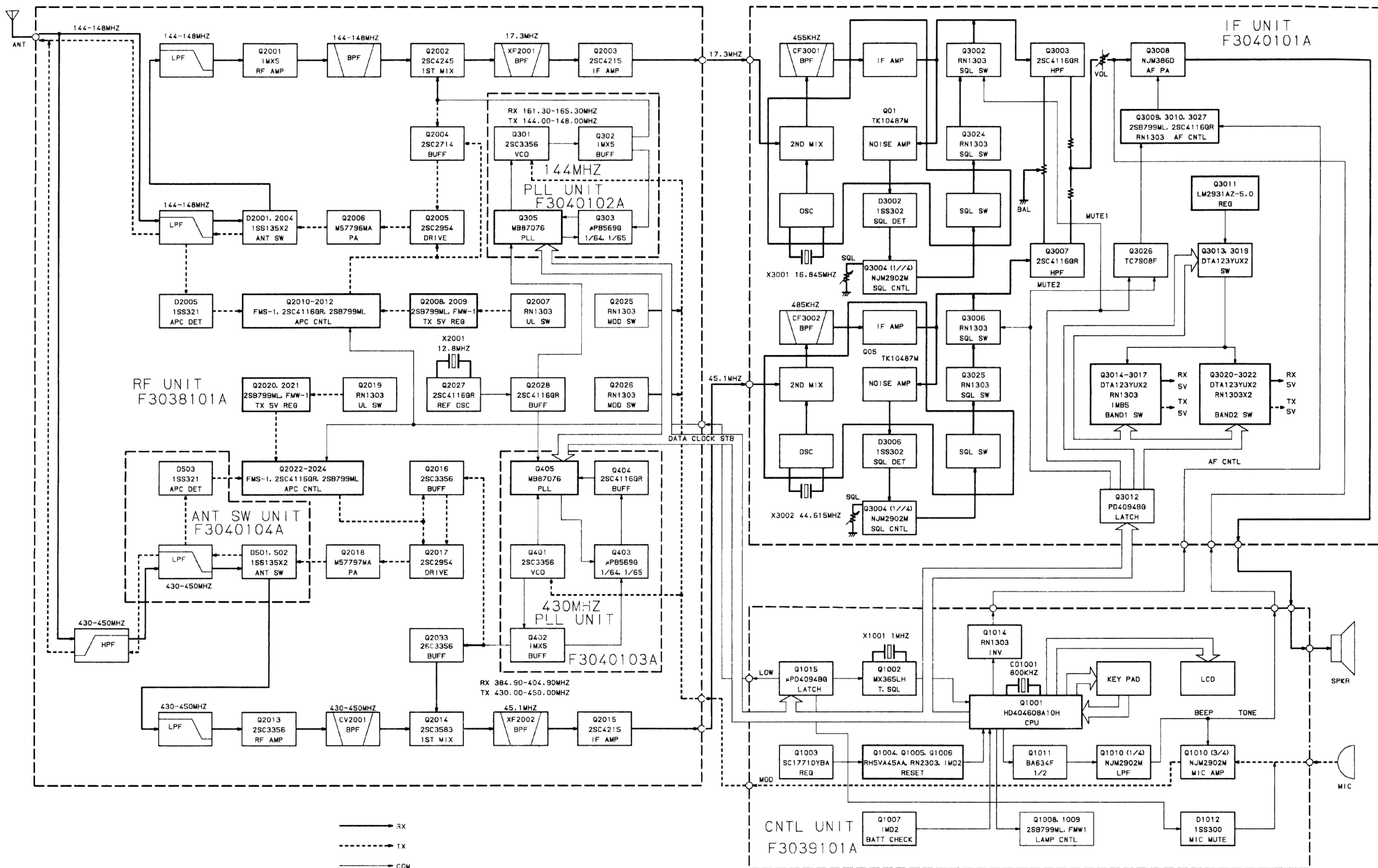
FT-470 BLOCK DIAGRAM
