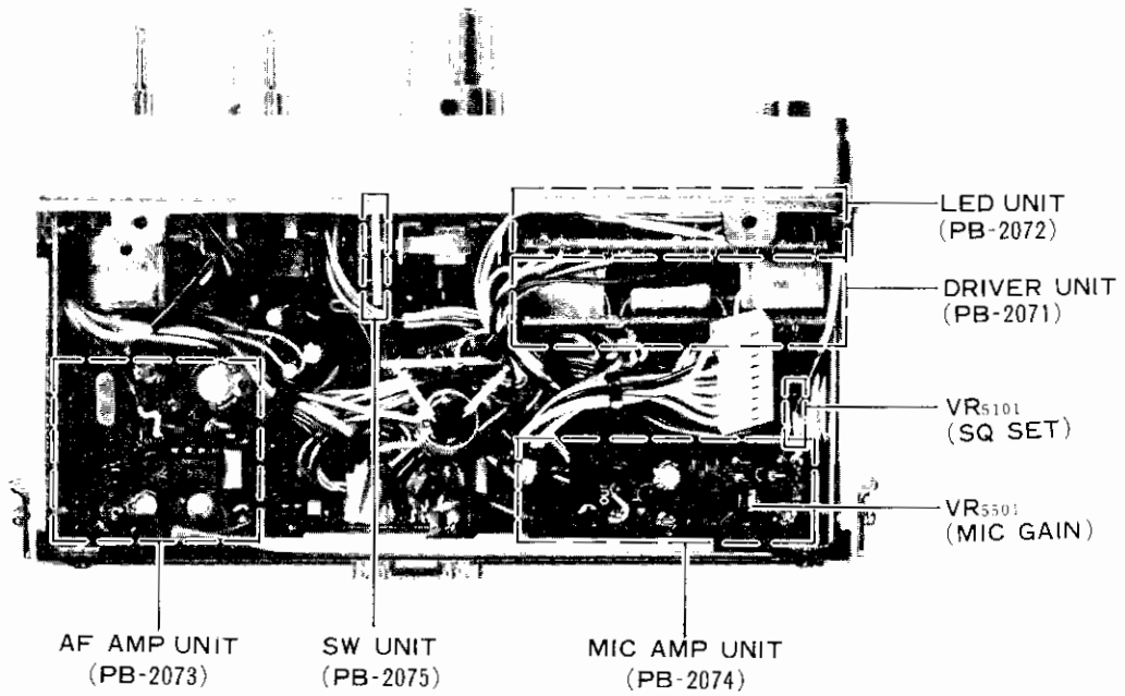
FT-720R BOTTOM VIEW
