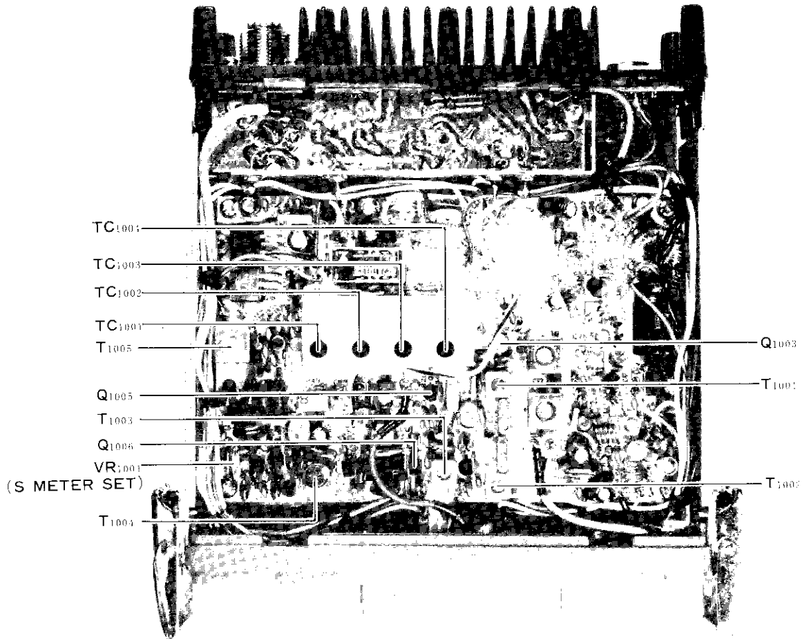
720RV RECEIVER SECTION ALIGNMENT POINTS
