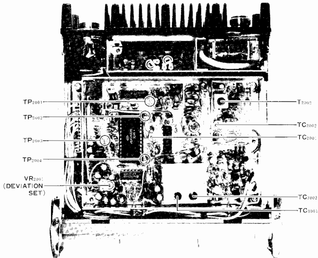
720RU PLL SECTION ALIGNMENT POINTS
