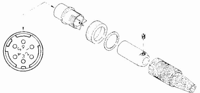
YM-32 MICROPHONE CONNECTIONS
