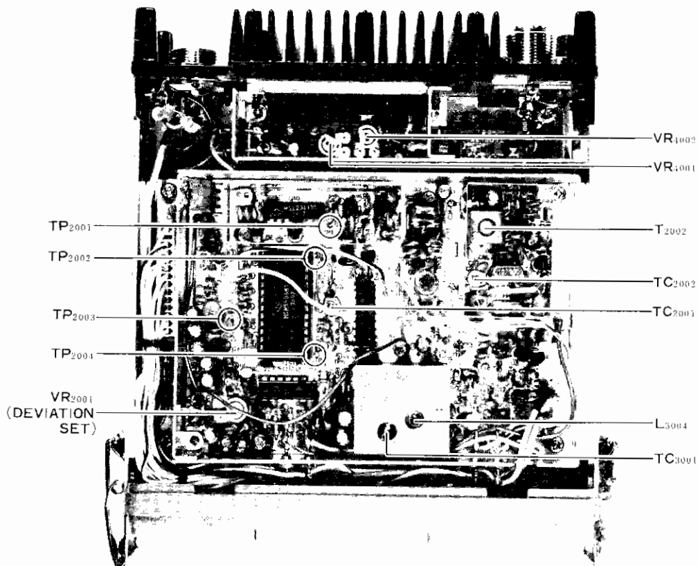
720RV PLL SECTION ALIGNMENT POINTS
