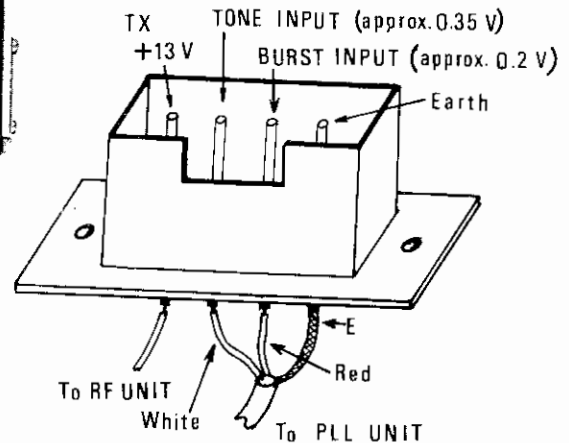
TONE IN CONNECTOR
