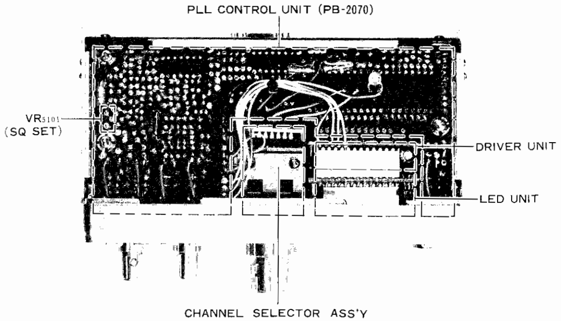
FT-720R TOP VIEW
