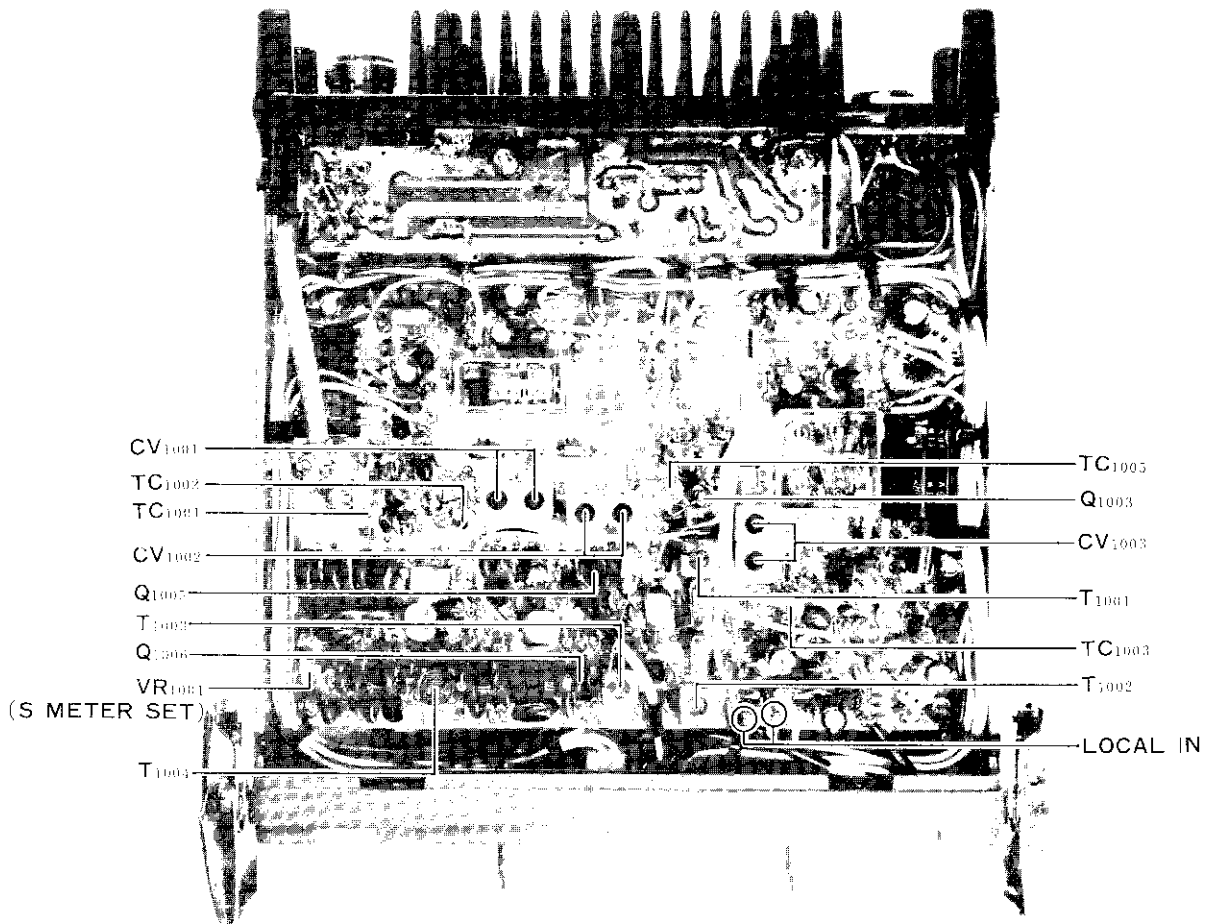
720RU RECEIVER SECTION ALIGNMENT POINTS
